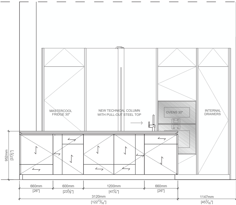
Elevation C
